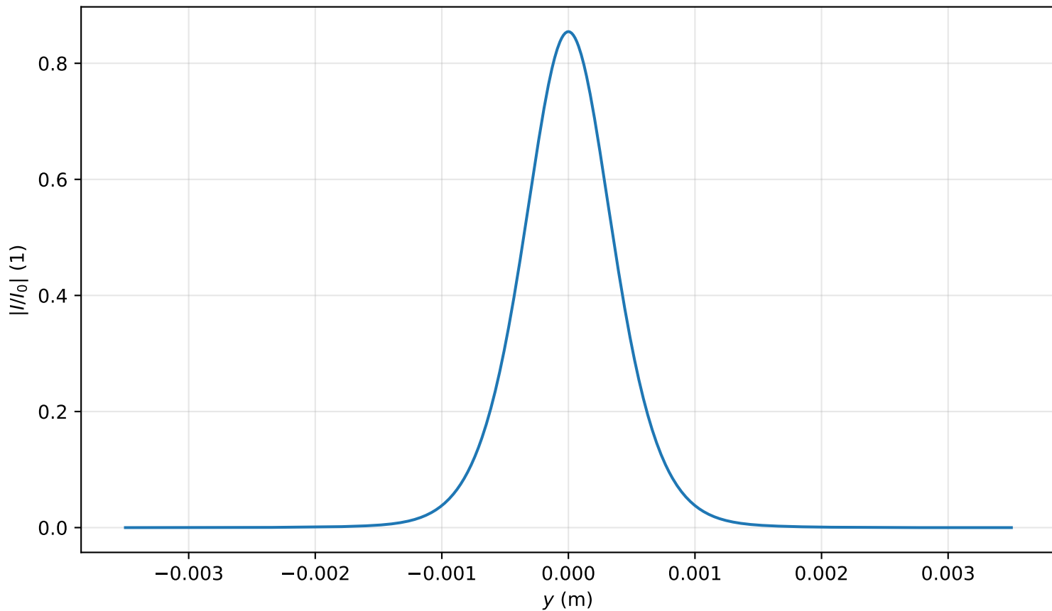
Intensity profile I(x=0, y, z=2.946)/I_0 , P_{in}=0.7P_{cr} , artificial time
